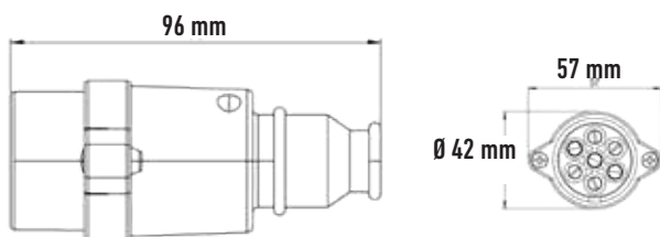
7 poled plug - ISO 1724
