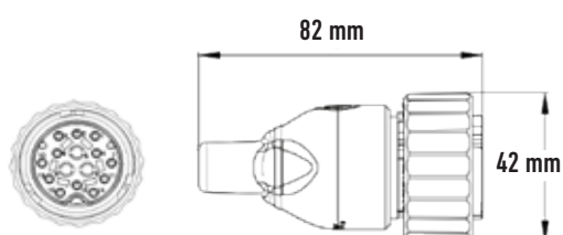
15 poled Bayonet plug
