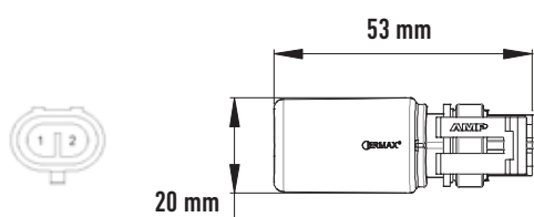
2 poled Super Seal plug
