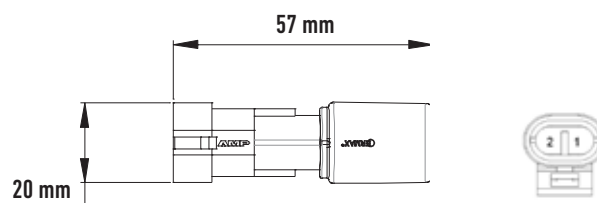
2 poled Super Seal socket
