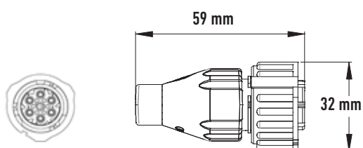
7 poled AMP 1.5 plug
