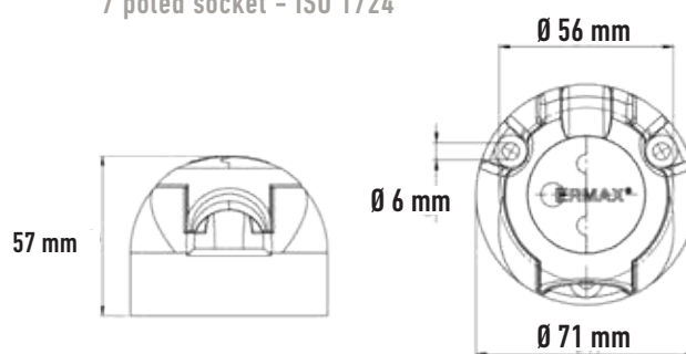
7 poled socket - ISO 1724
