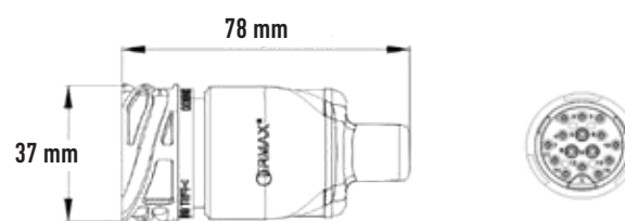
15 poled Bayonet socket
