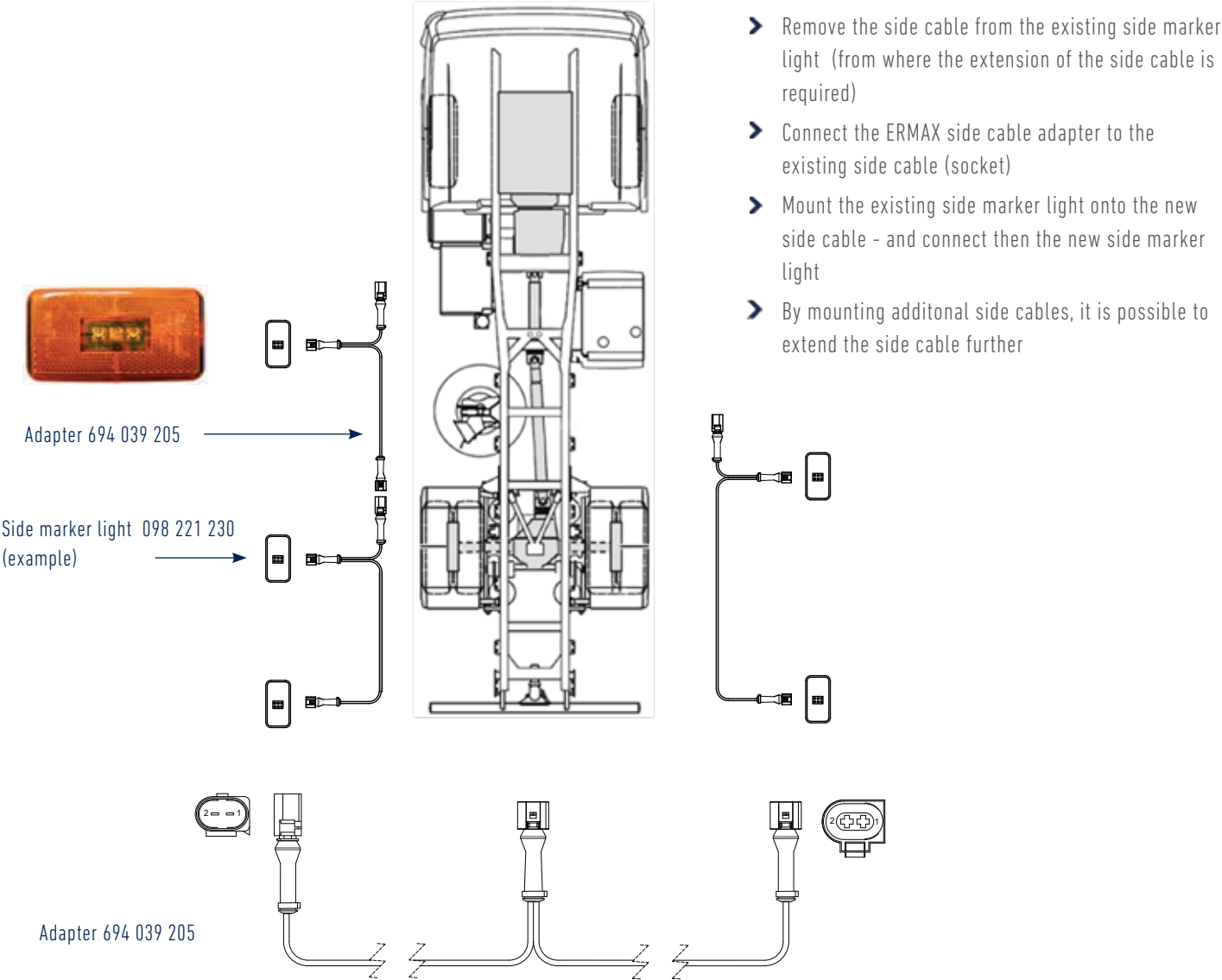
Side cable - Adapter SCANIA
